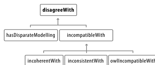
Figure 6: Taxonomy for the disagreement relations.
