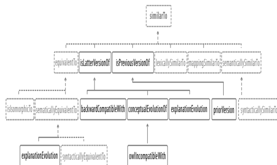
Figure 4: Taxonomy for versioning relations.
